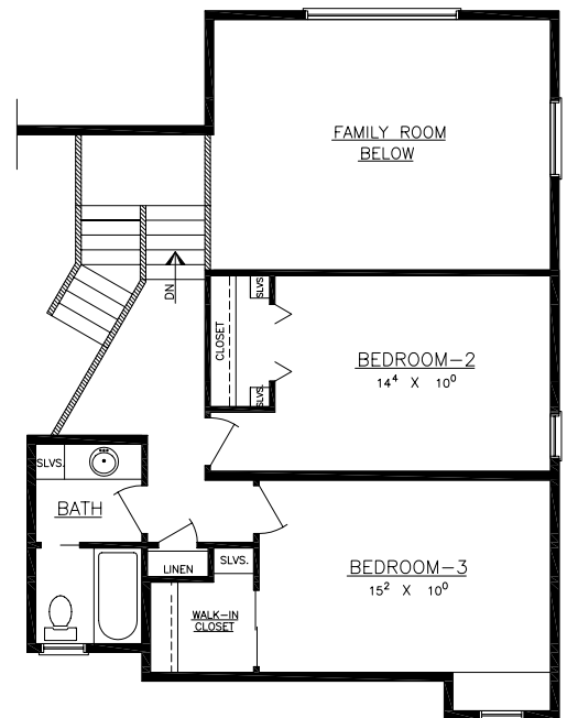
SECOND FLOOR AREA = 565 S.F.
